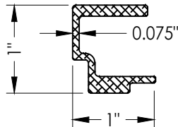
11 REINFORCEMENT Alum.
