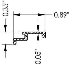
14 REINFORCEMENT Alum.
