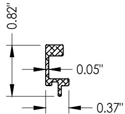
10 REINFORCEMENT Alum.
