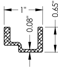
15 REINFORCEMENT Alum.
